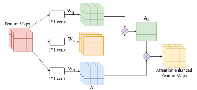
Fig. 2. The self-attention block architecture.
